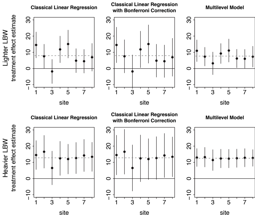
Figure 12.1 Estimates and 95% Uncertainty Intervals for Treatment Effects by Site and Birth Weight Group (Lighter and Heavier) Using Classical Linear Regression, Classical Linear Regression with Bonferroni Corrections, and a Multilevel Model
