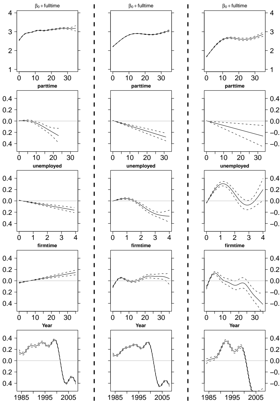
Figure 18.3 Fitted Dynamic Effects for High, Middle, and Low Educated Women (first, second, and third column respectively) Based on Model (18.13)
